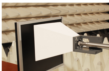
TEM horn in typical application
