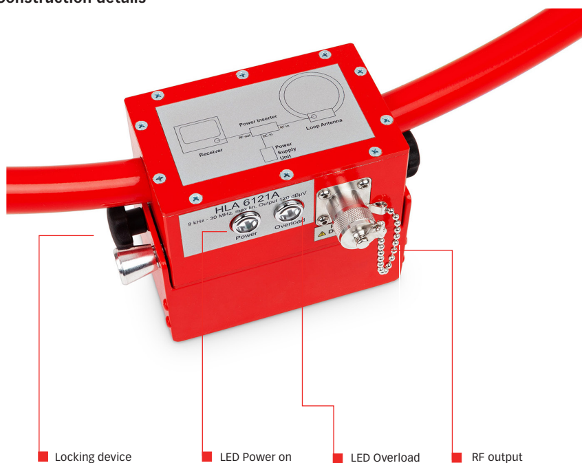
Construction details
